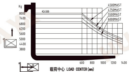
8.0T 载荷曲线图 8.0T load curve
