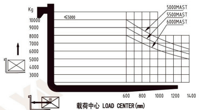
10T 载荷曲线图 10T load curve
